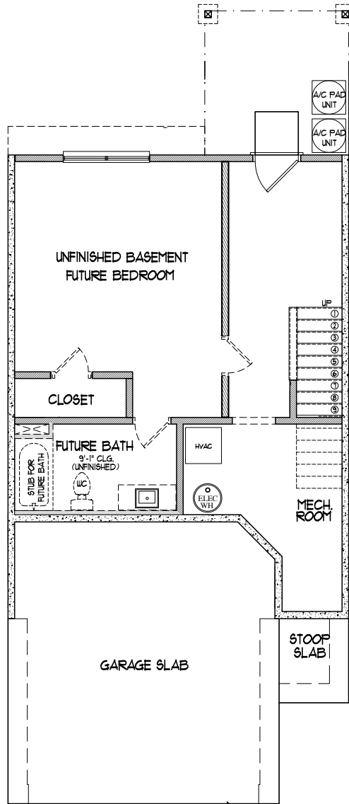
BASEMENT LEVEL W/ FUTURE BEDROOM
